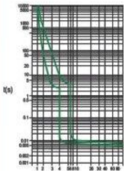
I In B curve
