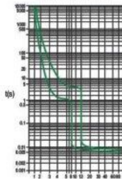
I In C curve
